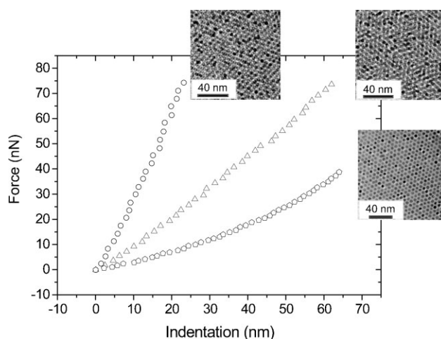
Figure 5. Force versus indentation curves of one (pentagon)-, two (triangle)-, and three (circle)-layer-thick Au nanoparticle membranes, all stretched across 2- \mu\text{m} -diameter holes. Insets: TEM detail images of the corresponding membranes.
