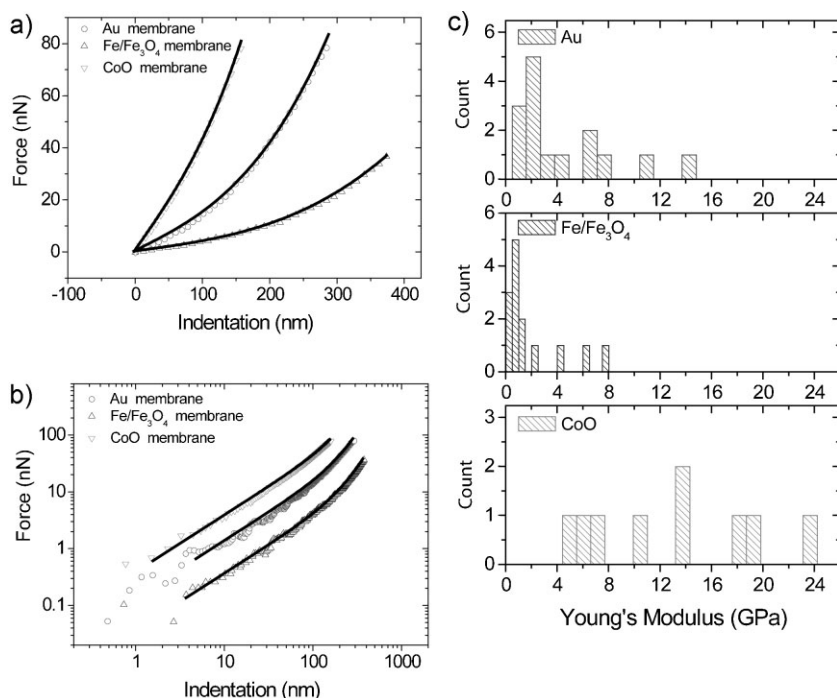
Figure 2. a) Representative force–indentation curves for Au, Fe/Fe 3 O 4 , and CoO nanoparticle monolayer membranes of diameter 10 μm. The black lines represent fits to Equation (1). b) Log–log plot of the data in (a). c) Histograms of Young's moduli E obtained from fits to Equation (1).
