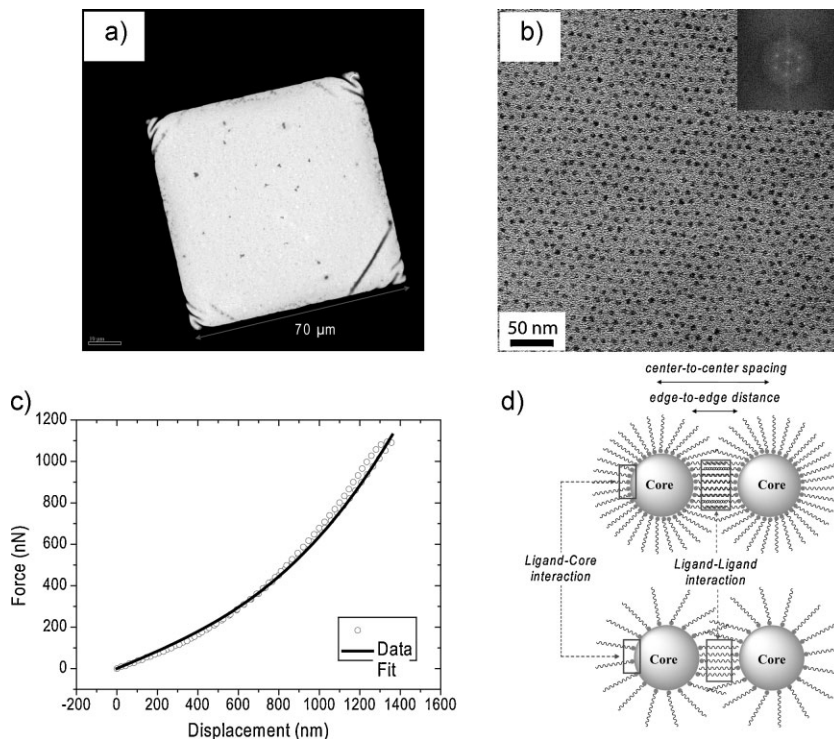
Figure 3. a) TEM image of a 70 \times 70\text{ }\mu\text{m}^2 freestanding membrane consisting of a monolayer of CoO particles. b) Higher-resolution TEM detail of the image in (a). Inset: the corresponding Fourier transform. c) Force-indentation curve taken with a blunt plateau tip (see Figure S5, Supporting Information). The black line represents the fitting curve using Equation (1). d) Schematic view of two interdigitated nanoparticles.
