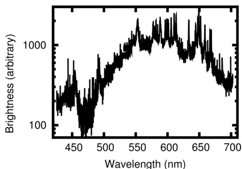
Fig. 1. Multiphoton fluorescence spectrum for \text{Ba}_9\text{Ag}_{10}\text{U}_4\text{S}_{24} (1064 nm excitation).
