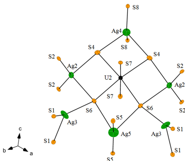
Fig. 5. Local coordination of atom U2 in the \text{Ba}_9\text{Ag}_{10}\text{U}_4\text{S}_{24} structure.
