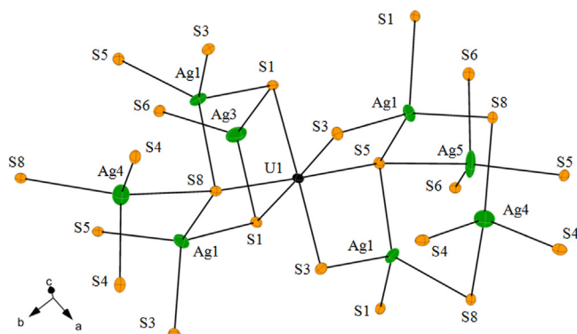
Fig. 4. Local coordination of atom U1 in the \text{Ba}_9\text{Ag}_{10}\text{U}_4\text{S}_{24} structure.
