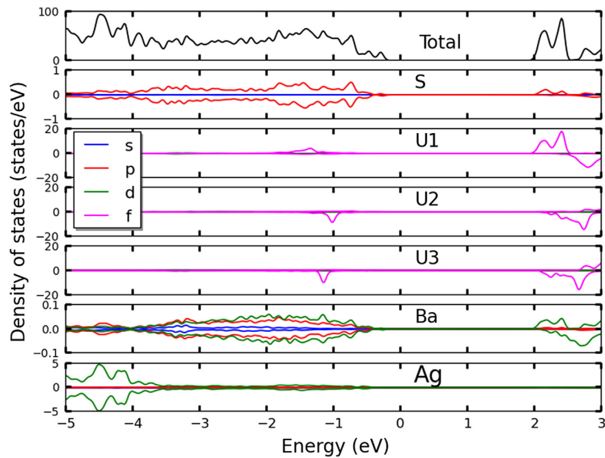
Fig. 7. Total (upper plot) and partial density of states (lower plots) of Ba 9 Ag 10 U 4 S 24 . For each atom, the PDOS is projected onto the relevant orbitals. The Fermi level is set at 0.
