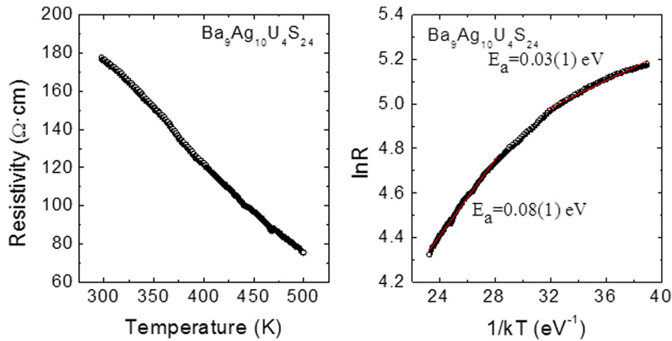
Fig. 8. Resistivity and the corresponding Arrhenius plots for Ba 9 Ag 10 U 4 S 24 .
