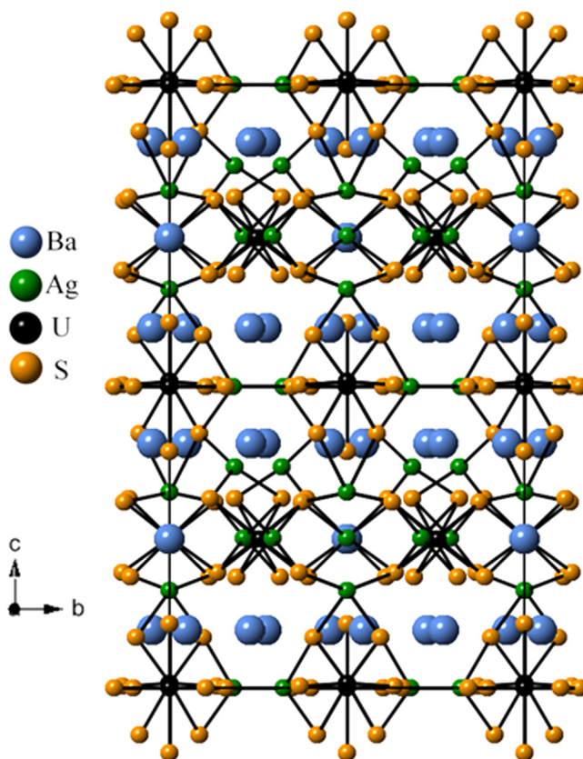
Fig. 2. General view approximately down the a axis of the \text{Ba}_9\text{Ag}_{10}\text{U}_4\text{S}_{24} structure.
