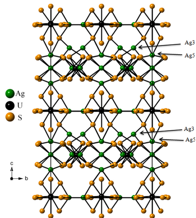
Fig. 3. The \text{US}_6 , \text{AgS}_4 , and \text{AgS}_3 networks in the \text{Ba}_9\text{Ag}_{10}\text{U}_4\text{S}_{24} structure.
